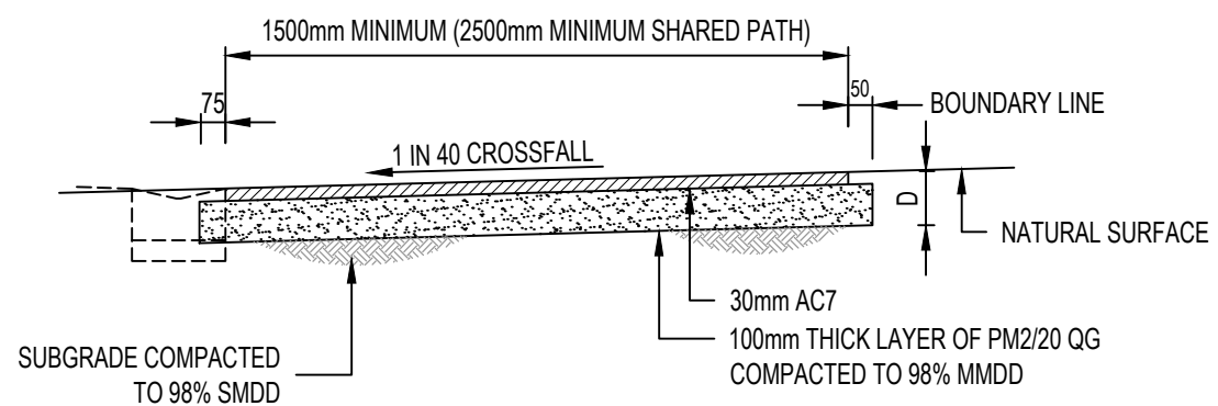
TYPICAL ASPHALT FOOTPATH SECTION
