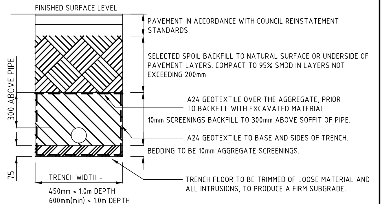
TYPICAL TRENCH AND BACKFILL - IN GROUNDWATER
