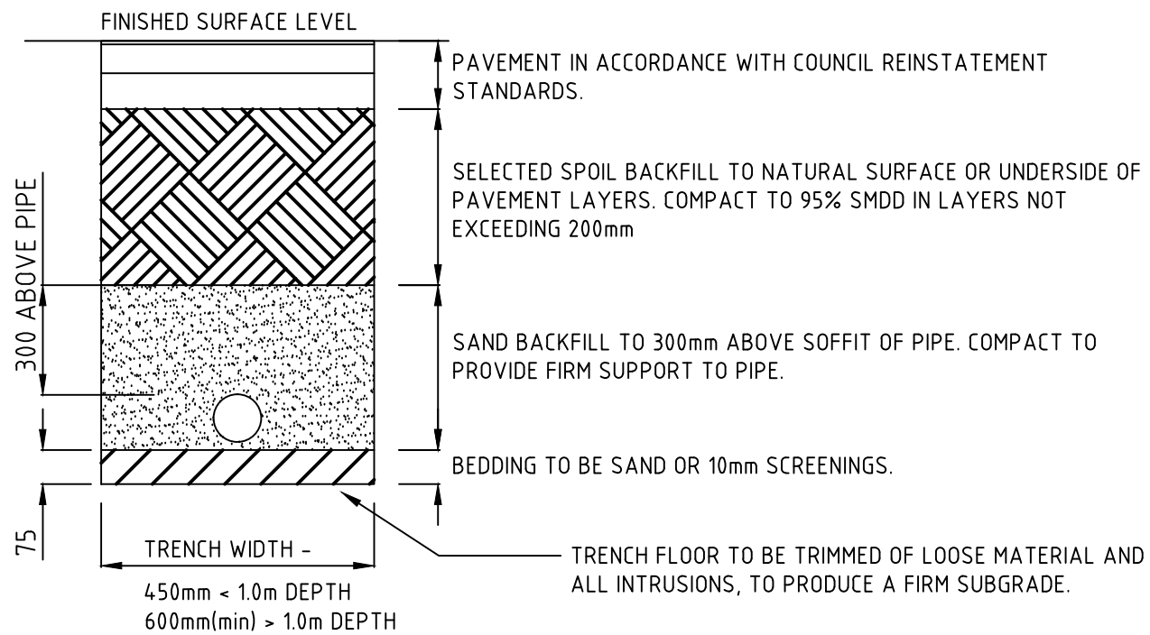
TYPICAL TRENCH AND BACKFILL - NO GROUNDWATER
